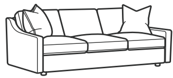
-31 SOFA 33H 83W 39D 19SH 77SW 24SD 22AH
